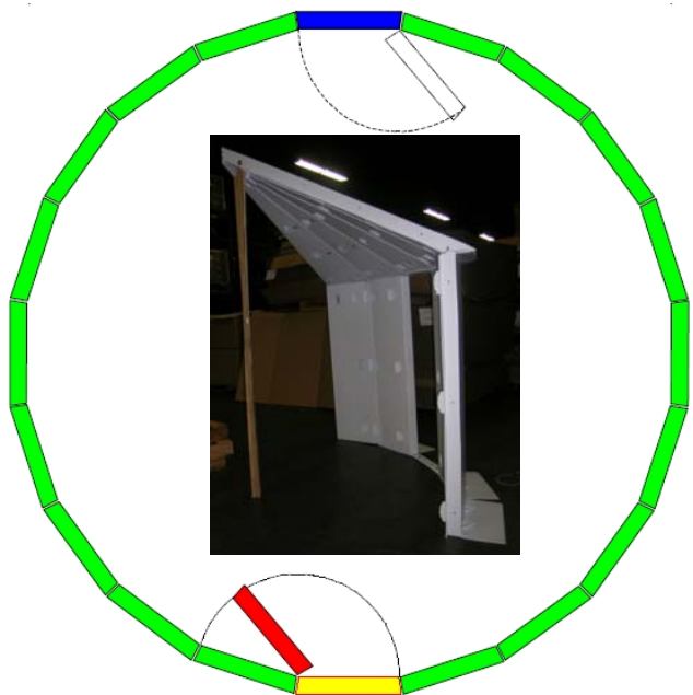
The standard TekYurt kit comes with a single Dutch-door and one window
