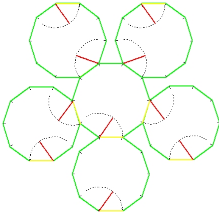
6-Room LiteYurt Structure
