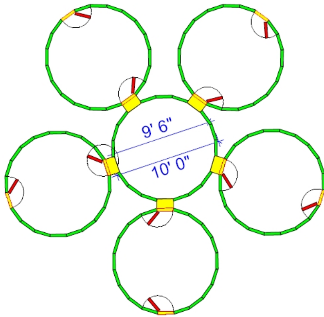
Six-Room Yurt Structure: 6 Yurts, 5 Connector Kits
