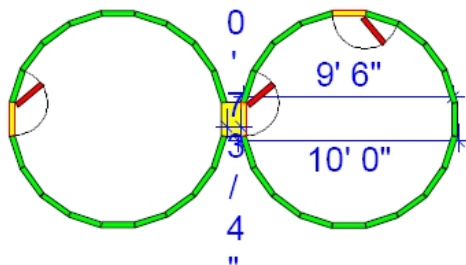
Two-Room Yurt Structure 2 Yurts, 1 Connector Kit
