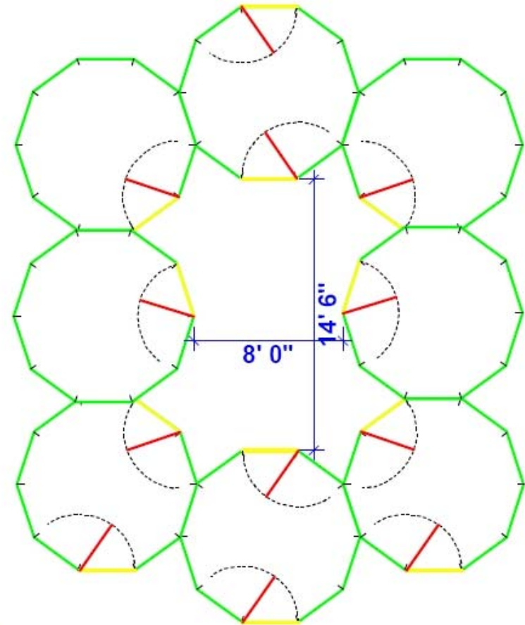
8-Room LiteYurt Compound
